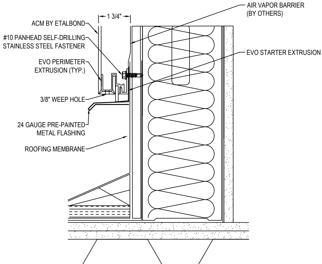
SECTION DETAIL
