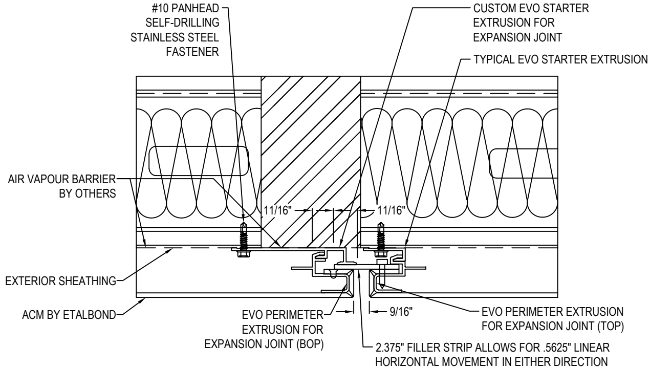
SECTION DETAIL
