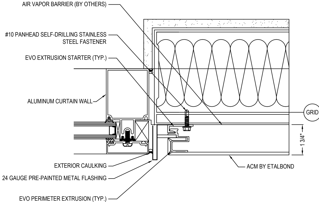
PLAN DETAIL
