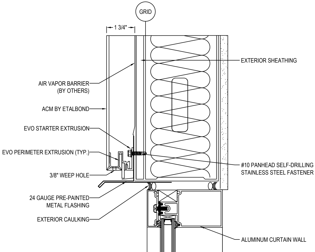
SECTION DETAIL
