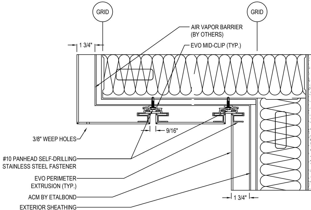
SECTION DETAIL
