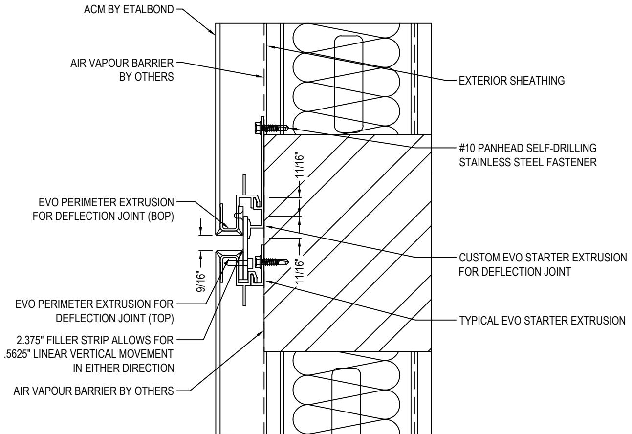
SECTION DETAIL
