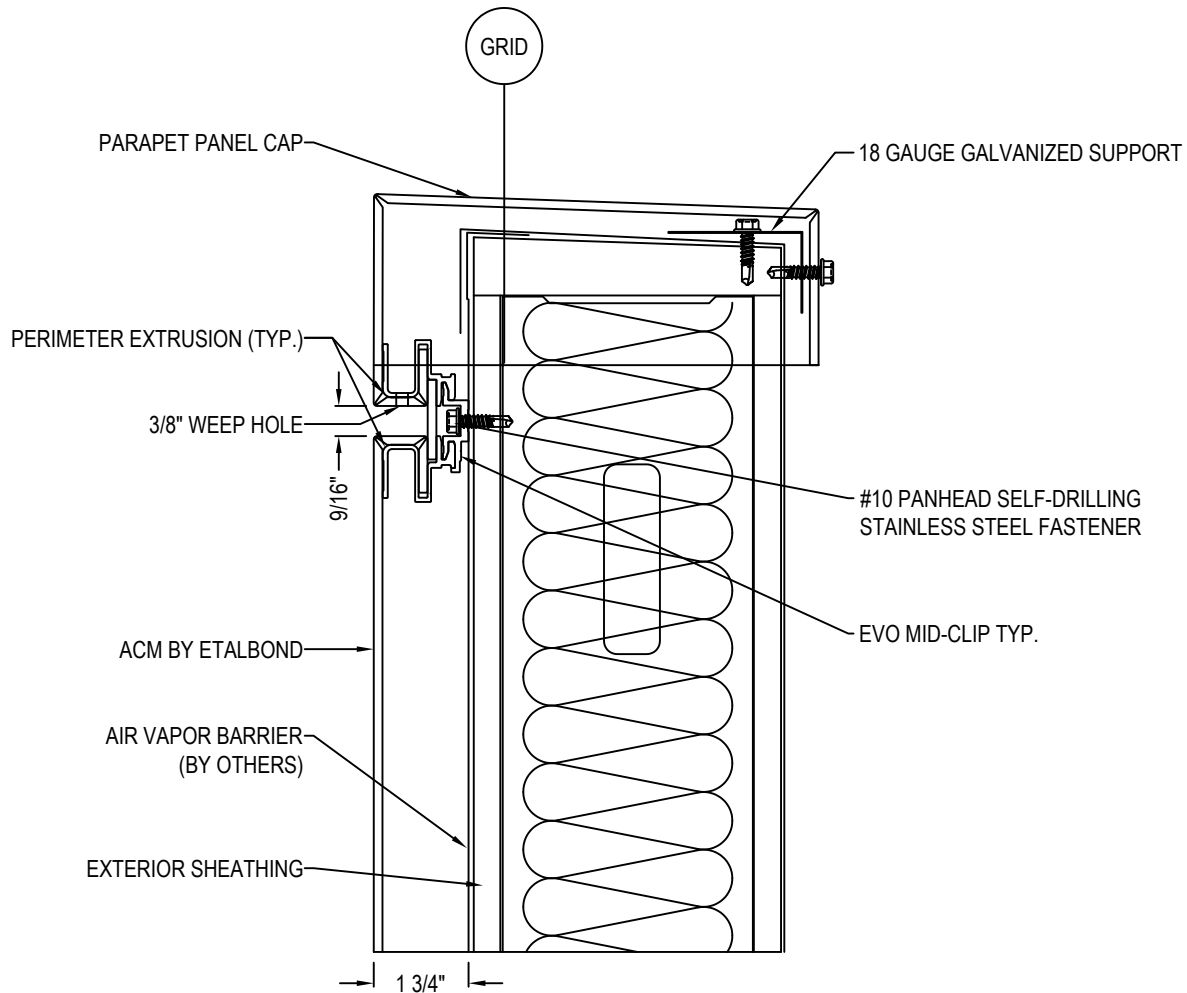
SECTION DETAIL
